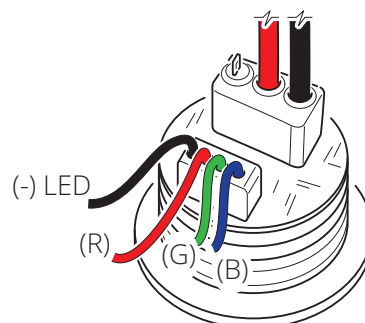
Single push + Single LED or RGB LEDs
