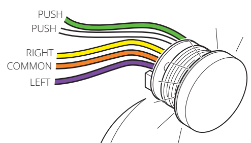
Triple push + 0-10 V + 2 LEDs
