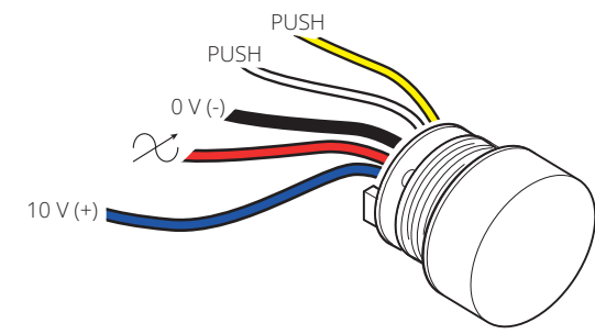
Single push + 0-10 V
