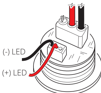
Single push + Single LED or RGB LEDs
