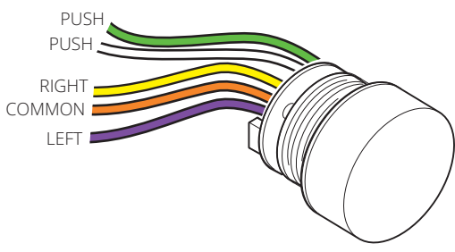
push + 0-10 V
