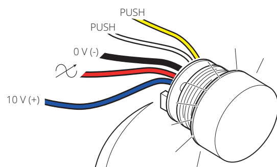
Single push + 0-10 V + 2 LEDs
